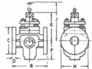
Sizes 1" - 6" Wrench operation
